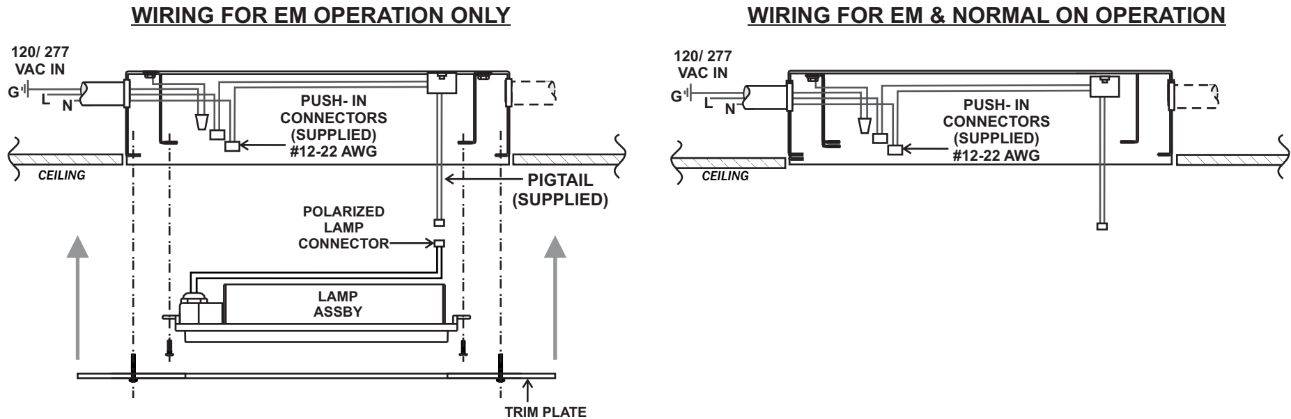
Fig. 4. RECESSED MOUNT- WIRING
