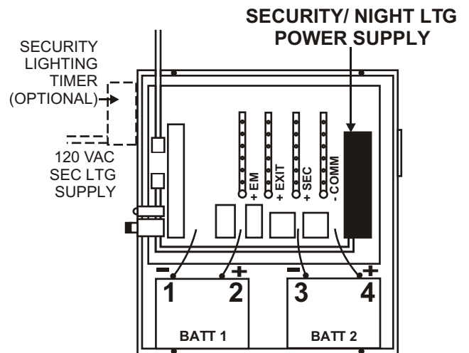
CENTRAL BATTERY PANEL (SERIES CBS)
